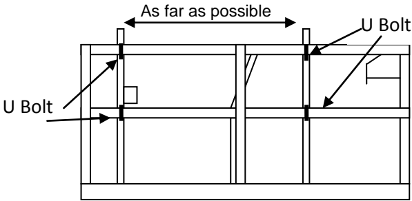
Figure 1.3 Sheet Handler attachment installation – Deck retracted
