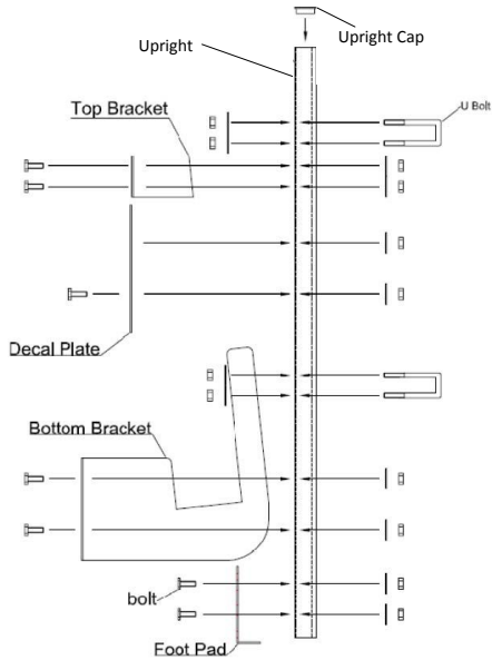
Figure 1.1: Sheet Handler Attachment assembly
